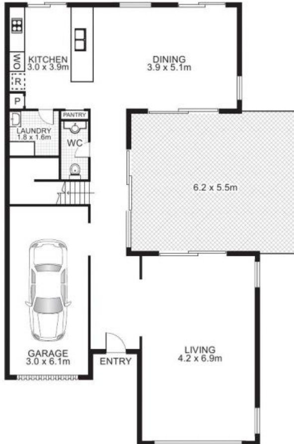
BOTTOM FLOOR
